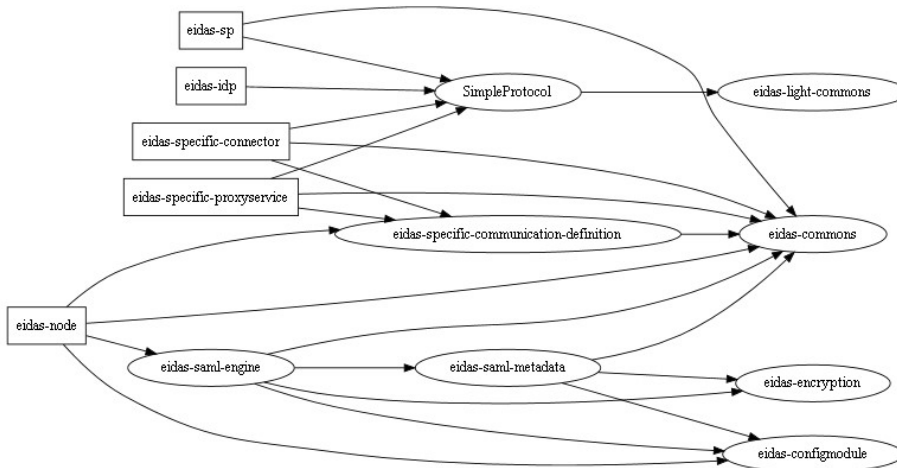
Figure 2: Component dependencies
